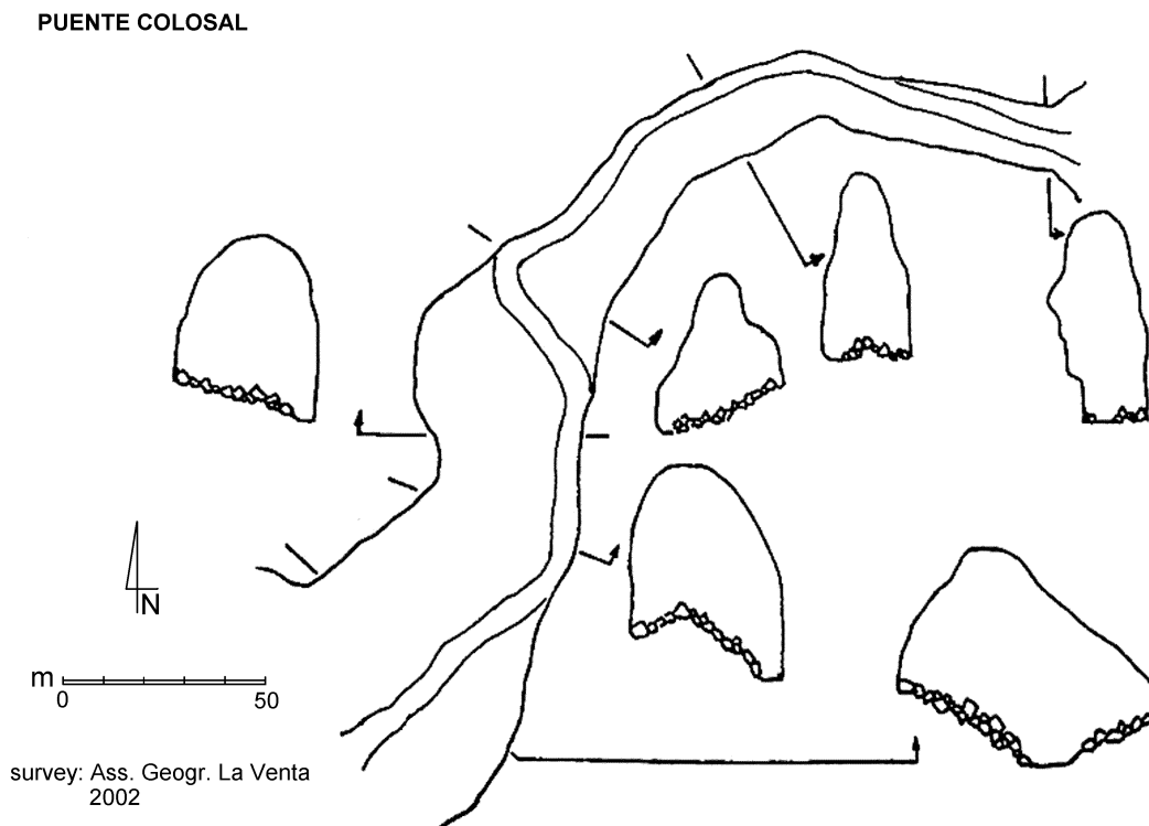
Fig. 6 – Plan view and cross-sections of Puente Colossal (survey: Ass. Geogr. La venta).
