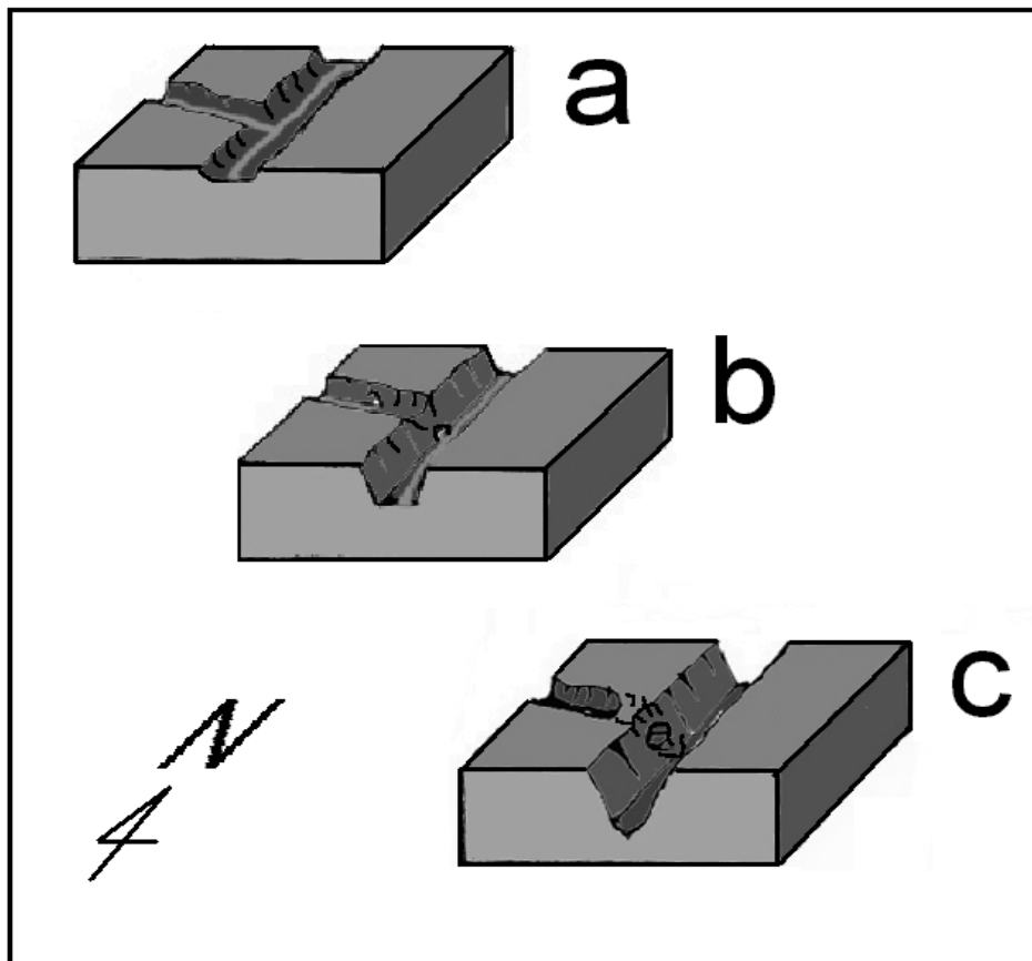
Fig. 13 – Hypothetical evolution steps of Puente Colosal (from: Livornese 2005)
