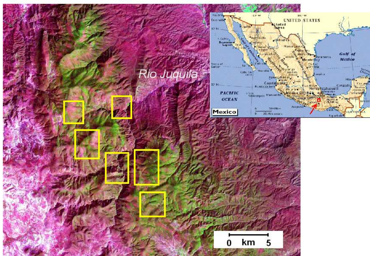
Fig. 1 – Location map and satellite image of Juquila Canyon. Yellow squares indicate investigated zones.
