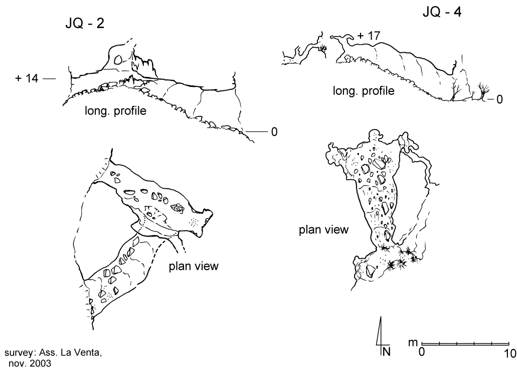
Fig. 3 – Plan views and longitudinal section of two paleo-phreatic caves located in the Juquila Canyon (survey: Ass. Geogr. La Venta).
