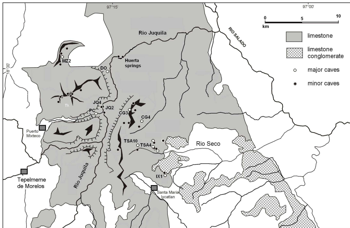
Fig 2 - Map of the Juquila karst area, showing the location of caves. Cave indexes as in Appendix (from: Geological Map of Mexico – INEGI).
