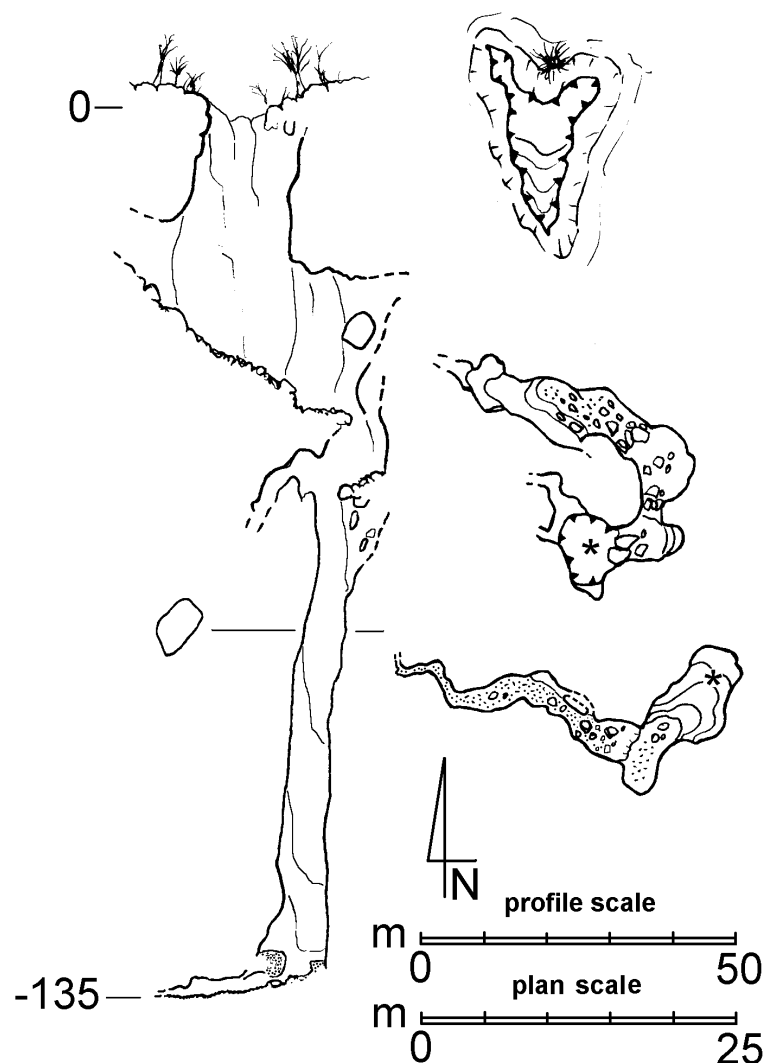
Fig. 11 - Plan views and longitudinal section of two caves in the Llano la Cumbre, S. Maria Ixcatlan (survey: Ass. Geogr. La Venta).
