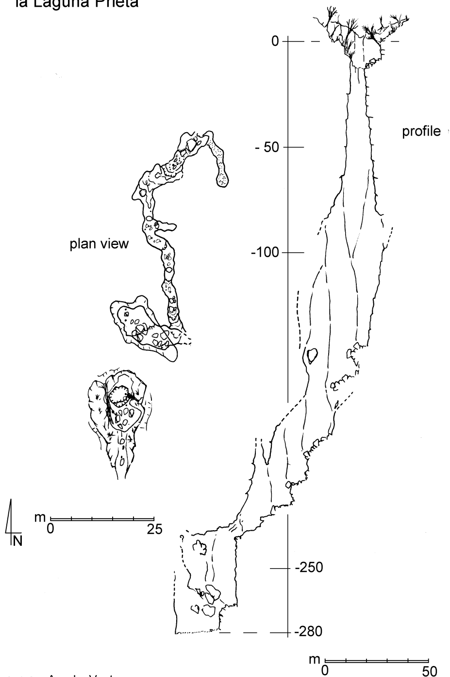
Fig. 9 - Plan views and longitudinal section of Pozo de la Laguna Prieta, Cerro Grande (survey: Ass. Geogr. La Venta)
