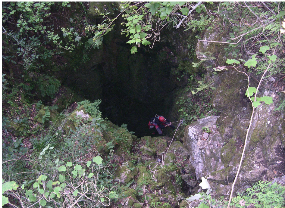
Fig. 8 – The entrance pit of the Pozo de la Laguna Prieta, Cerro Grande (photo: Ass. Geogr. La Venta).
